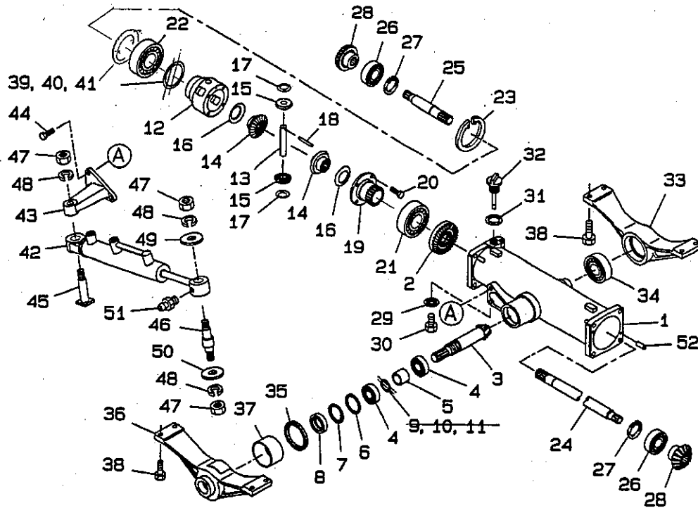
FIG.211 REAR DIFFERENTIAL
