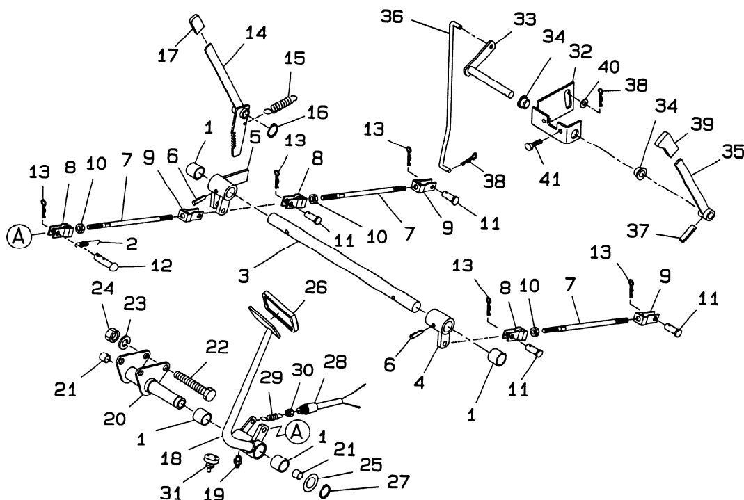
FIG.217 BRAKE & 4WD CONTROL LINKAGES
