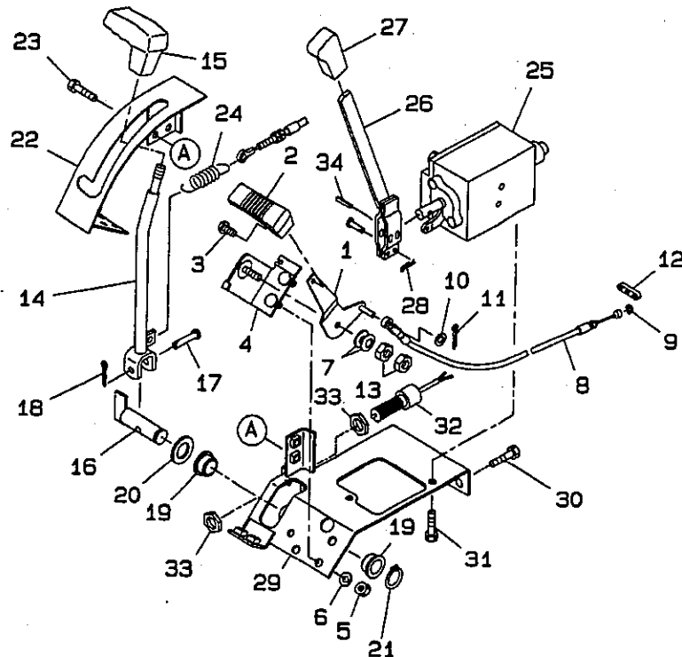
FIG.213 PTO,HPL, AND ACCEL CONTROLS
