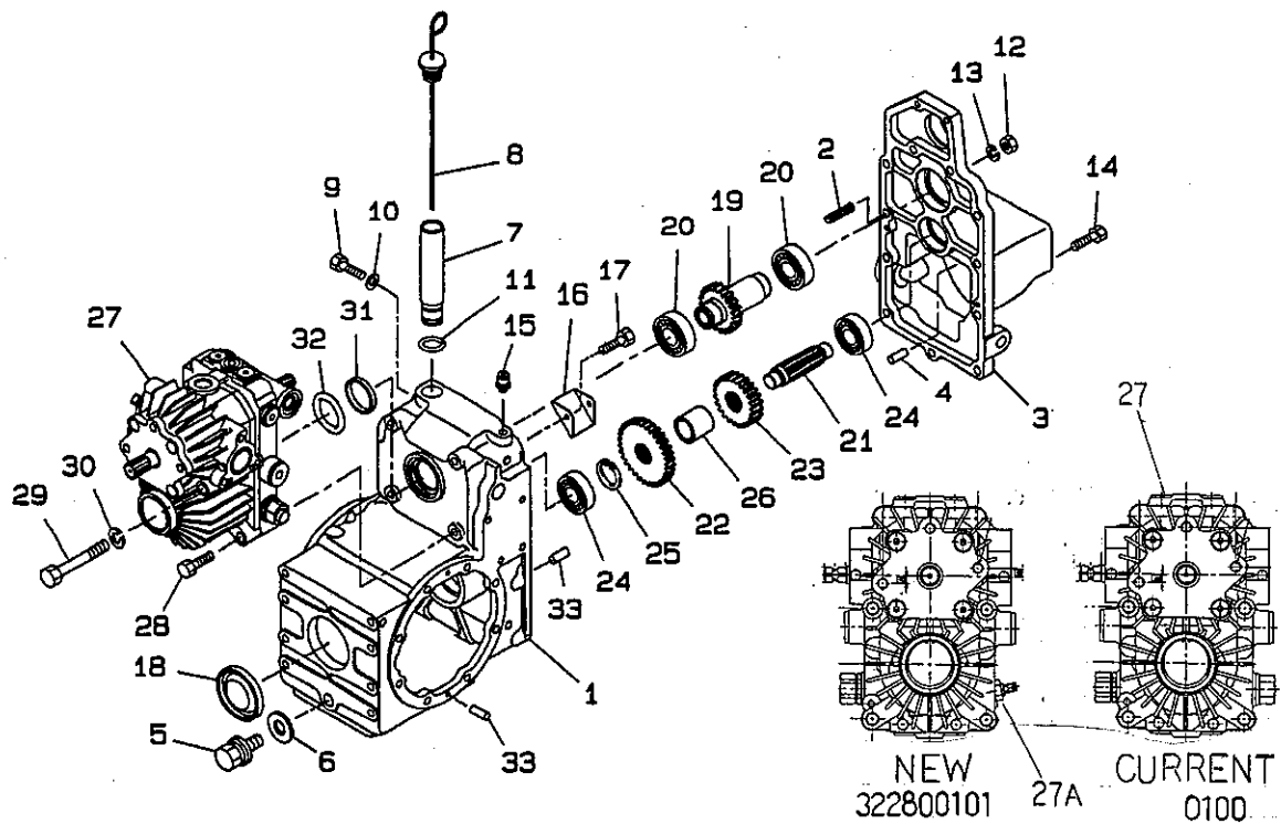
ミツシヨ FIG.208 TRANSMISSION
