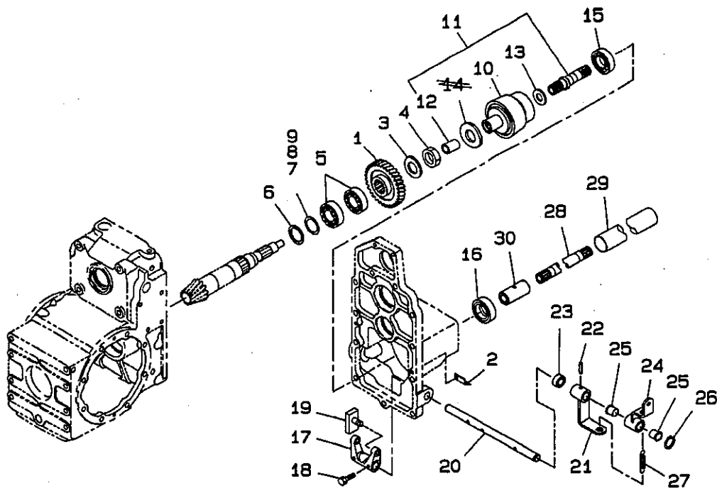
ミツシヨ FIG.209 TRANSMISSION
