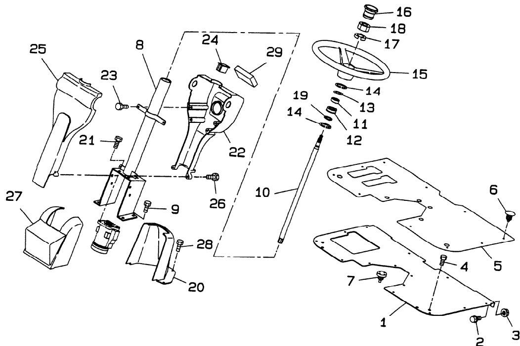
FIG.225 STEERING,DASH BOARD AND STEP
