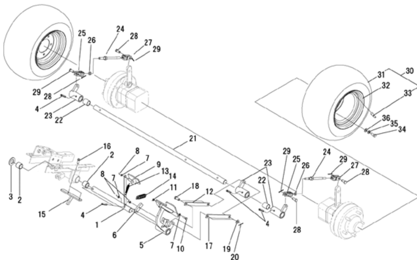
BRAKE、FRONT WHEEL
