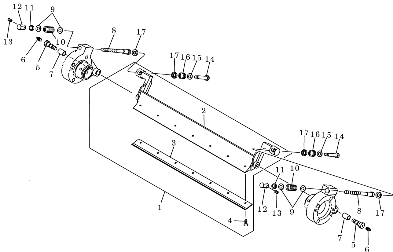
BED KNIFE
